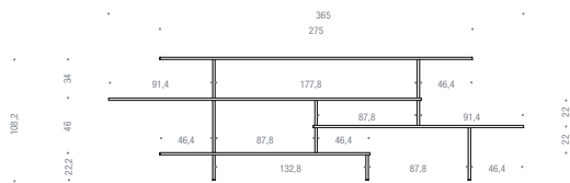
COMPOSITION B L365 D40 H108,2
