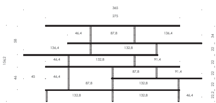
COMPOSITION H L365 D40 H156,2
